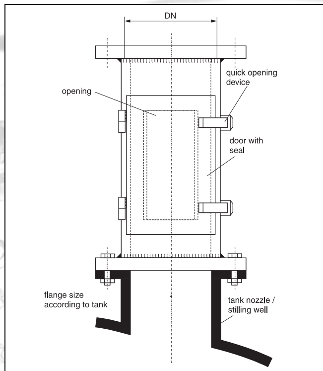
Calibration Chamber and Sample Hatch
