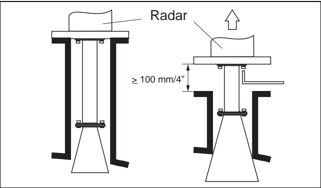
Antenna extension
