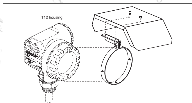
Weather Protection Cover
