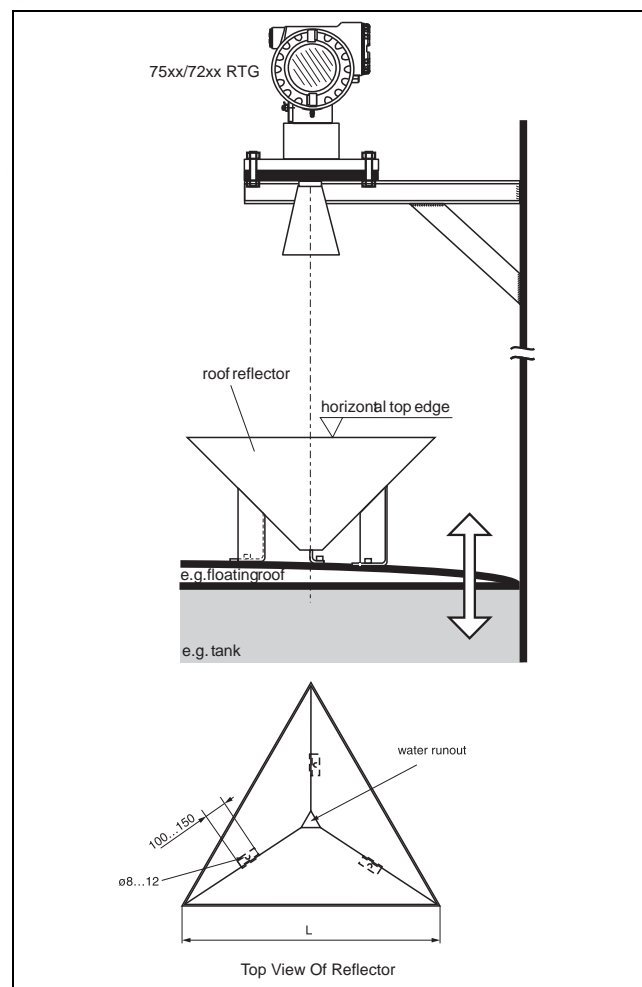
Roof Reflector
