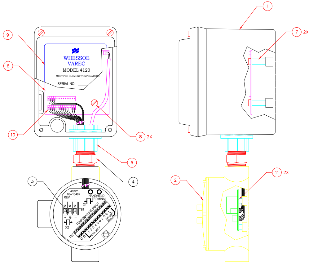
Figure 8 Model 4120 Component Identification
