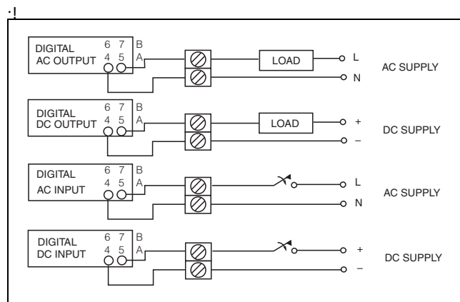
Discrete Inputs and Outputs
