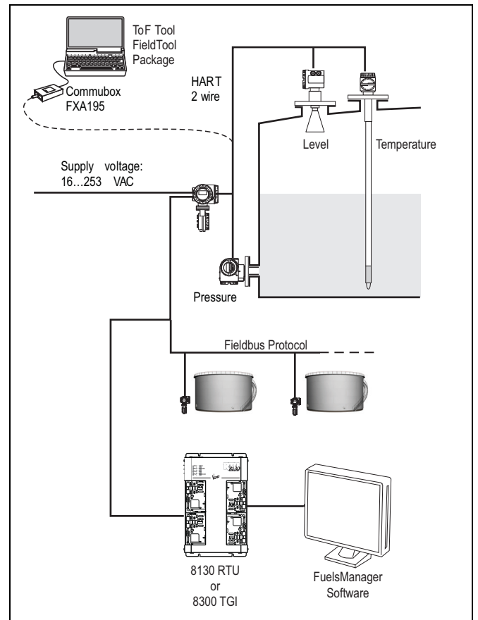
Example System Diagram
