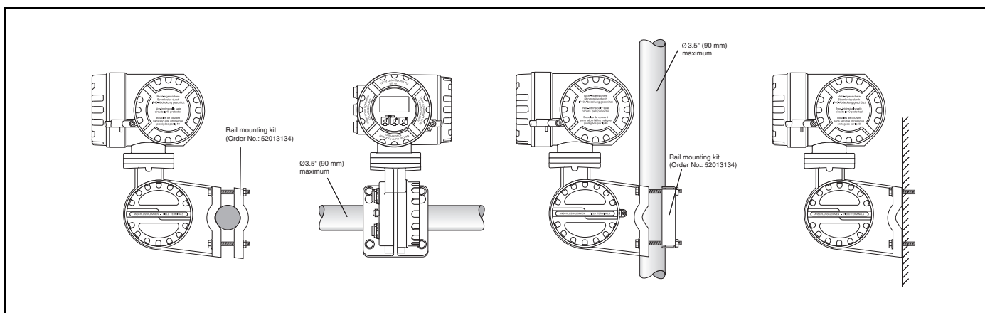
Typical 4590 TSM Installation & Mounting Methods
