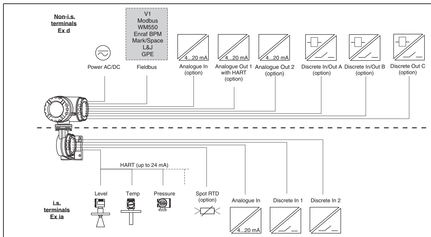
Instrument connections for the 4590 TSM
