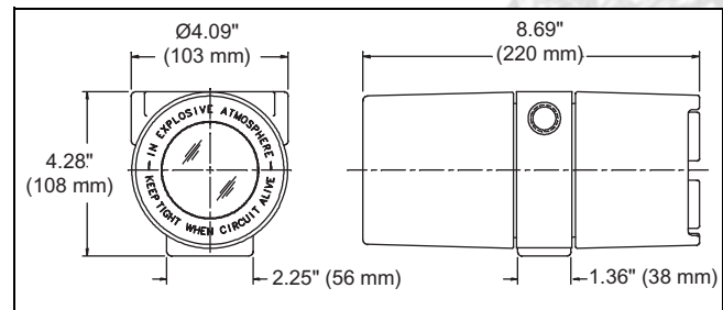
4200 MFT Dimensions
