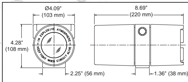
4200 MFT Dimensions
