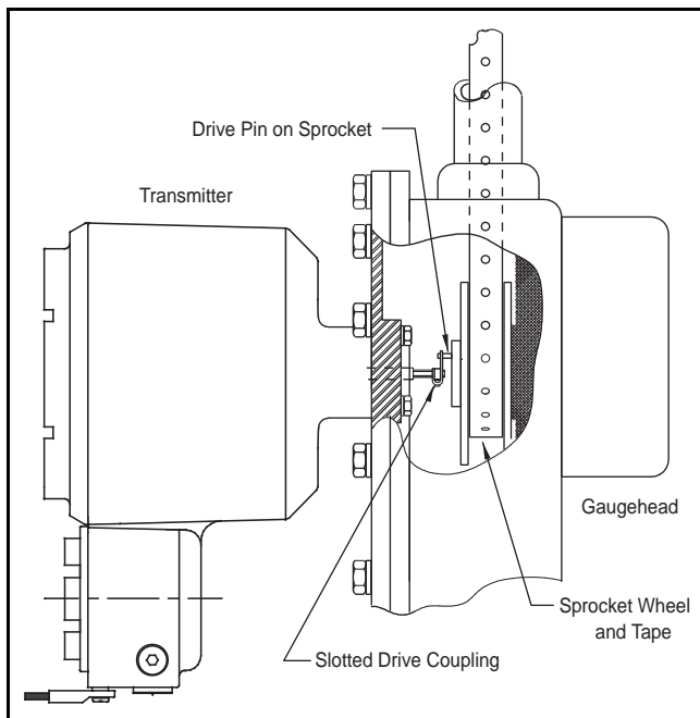
4110 HLE connected to a 2500 Automatic Tank Gauge (ATG)
